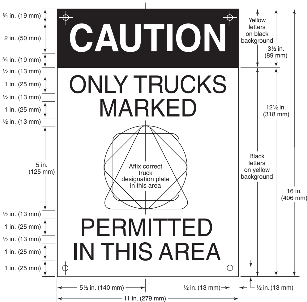
FIGURE 8.4.2.1 Building Sign for Posting at Entrance to Hazardous Areas.
